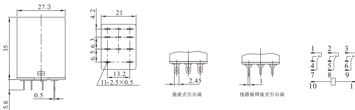
HHC68B-3Z(HH53P)
