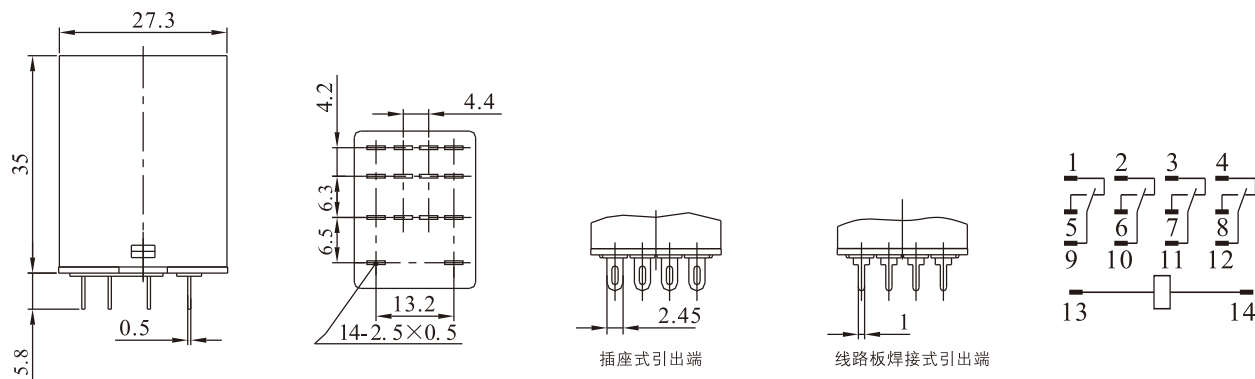
HHC68B-4Z(HH54P)
